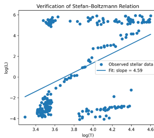
Figure 2: Log–log Plot of Stellar Luminosity Versus Effective Temperature
