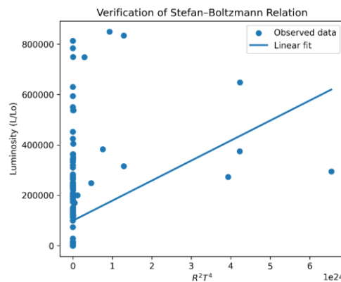
Figure 3: The scatter plot of luminosity ( L/L_{\odot} ) versus R^2T^4
