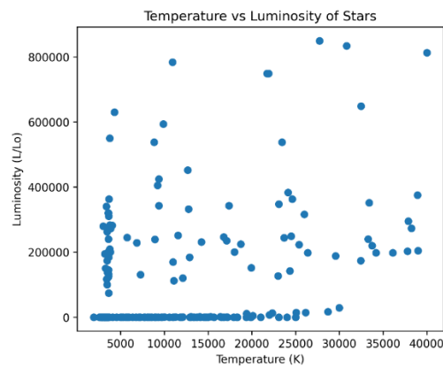
Figure 1: Scatter Plot of the Surface Temperature of the Stars Against Luminosity
