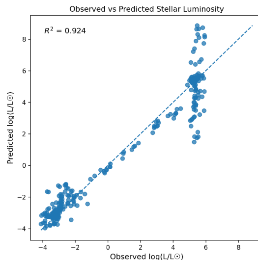
Figure 6: Observed vs Predicted Luminosity
