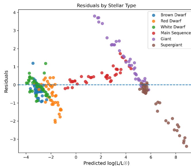
Figure 7: Residual Analysis of Predicted and Observed Luminosity for Different Stellar Types
