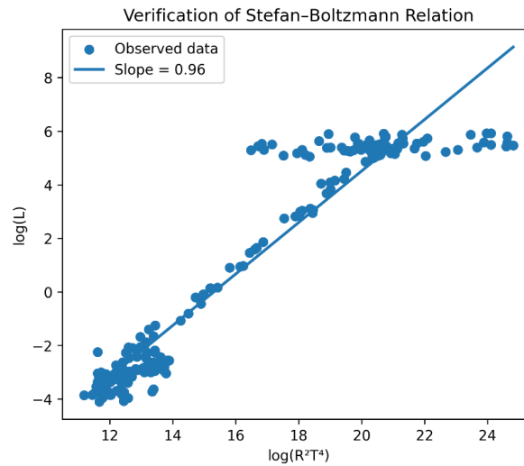
Figure 4: The Scatter plot of the Logarithmic Values of L and R^2T^4
