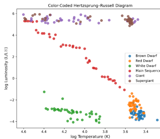
Figure 5: Scatter Plot of Stellar Log Luminosity ( L/L_{\odot} ) Versus Log Temperature T
