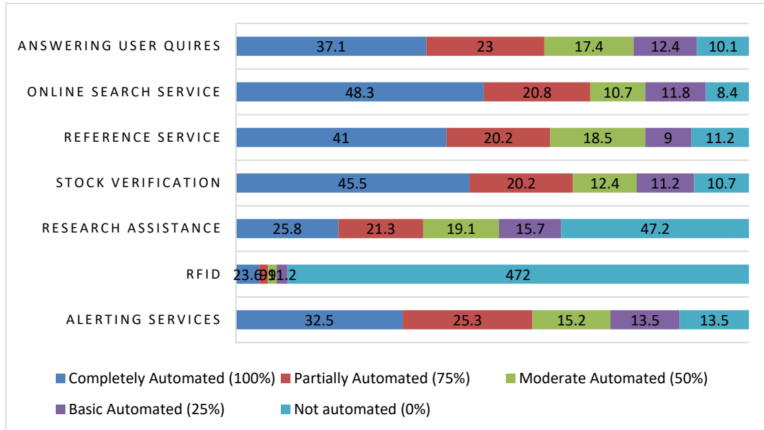
Figure 4: Services Automated
